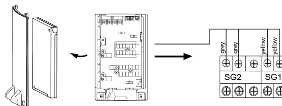
Fig. 9: Raccordement SG1/SG2
